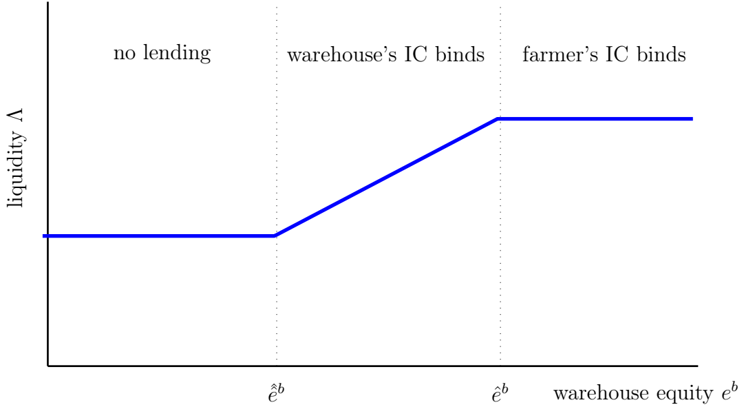
Figure 2: The graph depicts the liquidity multiplier \Lambda as a function of warehouse equity as analyzed in Subsection 4.4.
