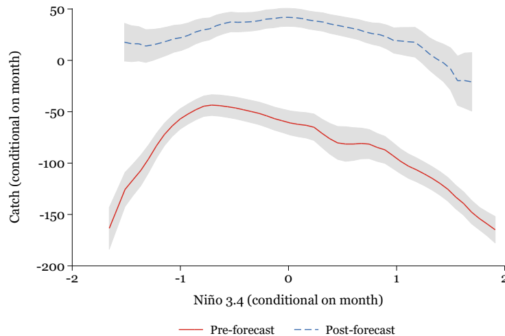
Figure 1: Output and ENSO before and after forecasts
