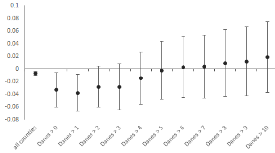
Figure A4: Coefficients on interaction between year 1870 and \ln(\text{Danes1880}) for different subsamples (based on the number of Danes in 1880), dependent variable: \ln(\text{cows}) .
