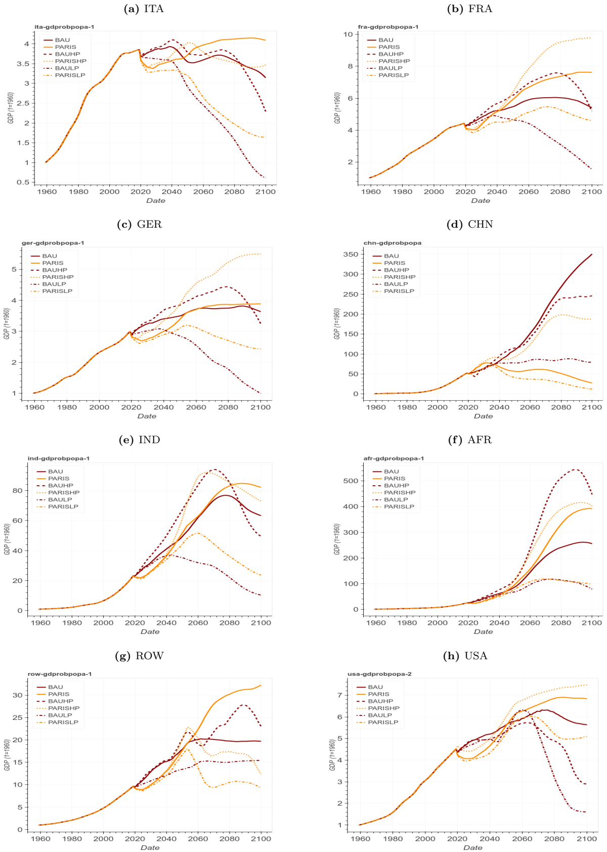
Figure 11: GDP levels - Robustness - population
