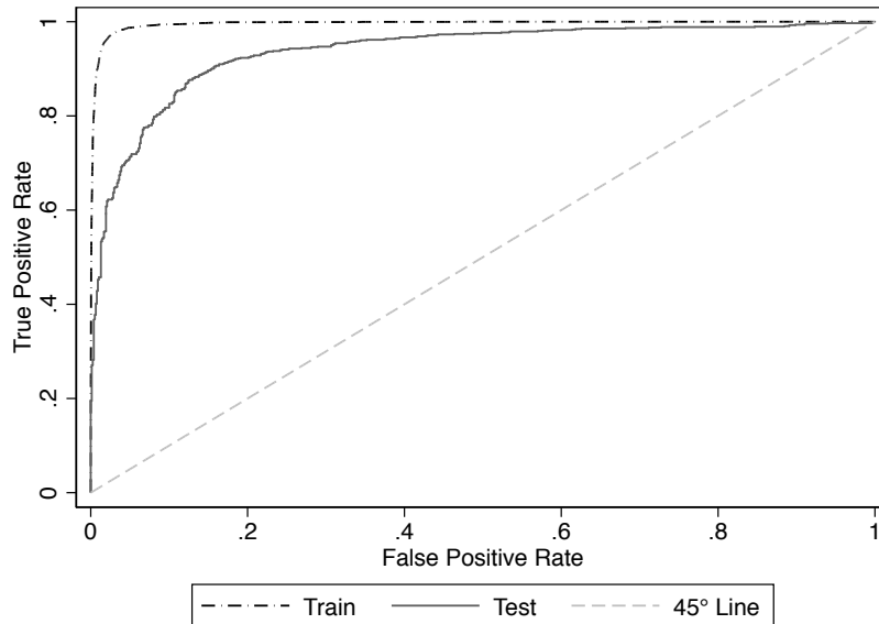
Figure A.1: ROC Curves for Post-Detection CNN
