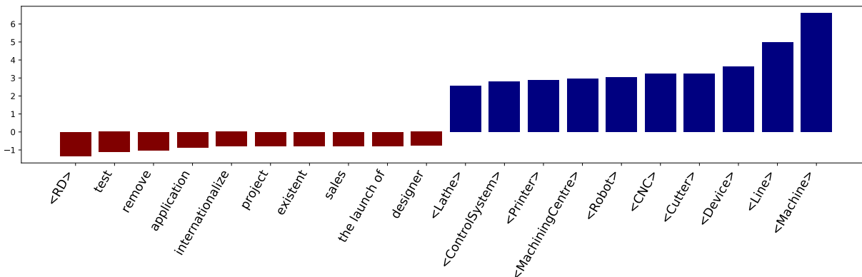
Figure E1: Predictive Features for Technology in the Text Data.
