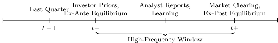
Figure 4: Model Timeline
