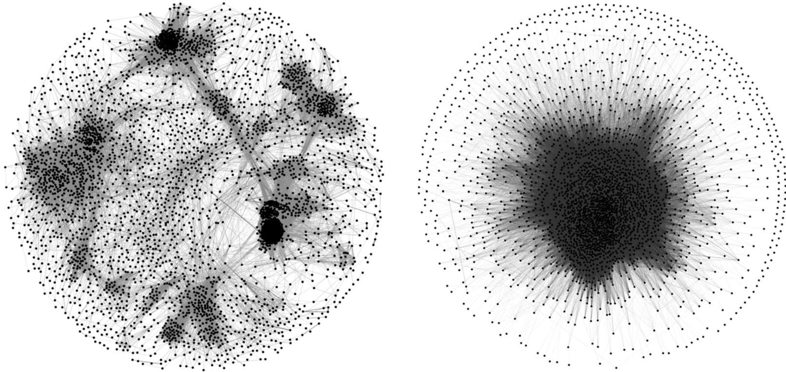
FIGURE 2: NETWORK VISUALIZATION
