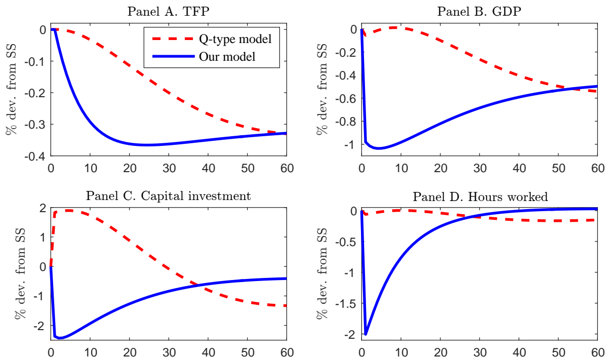
Figure A2: Impulse responses to an adverse financial shock in the Q-type model and ours
